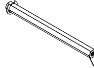
Stainless Steel REX Shaft 8mm Diameter, 96mm Length SKU: 2106-4008-0960 QTY: 4
