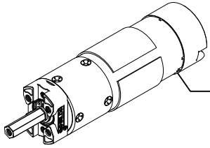
5203 Series Yellow Jacket Planetary Gear Motor 19.2:1 Ratio SKU: 5203-2402-0019 QTY: 4
