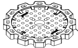
Track Sprocket, 12 Tooth SKU: 2401-0014-0012 QTY: 8 (four 2 packs)
