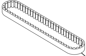
5mm HTD Pitch Timing Belt 9mm Width, 320mm Pitch Length SKU: 3412-0009-0320 QTY: 2
